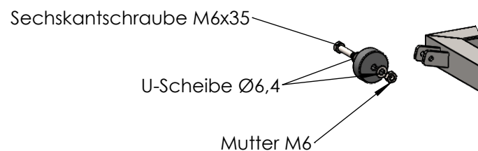
DETAIL C
