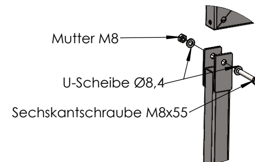
DETAIL B
